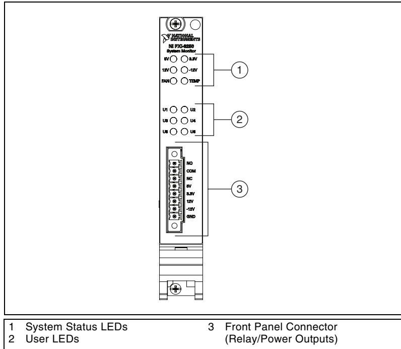
Figure 3-2. NI PXI-8250 Front Panel Diagram
